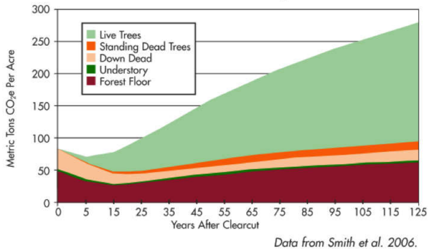
Figure 5. Non-soil forest carbon in a spruce-fir stand, northeastern USA. 61
