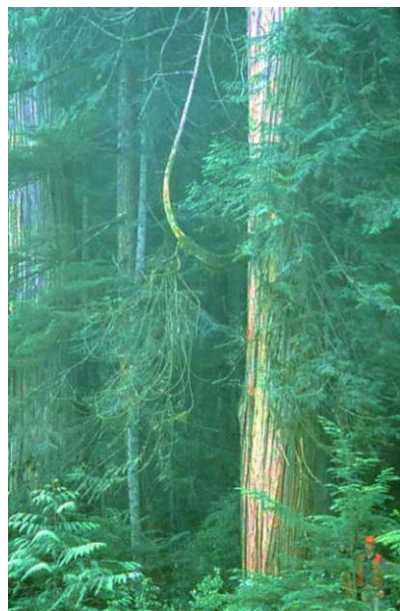
Figure 16. Old-growth cedar-hemlock forest, northern Vancouver Island. A. Inselberg
